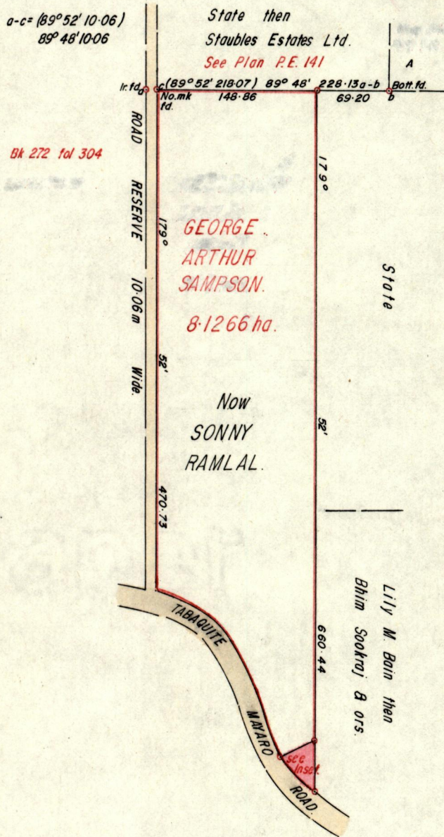
N.B. Tabaquite Mayaro Road. Scaled from Bk. 272 fol 304
